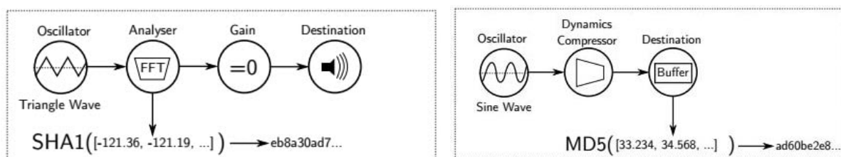
➤ Figura 3: Métodos AudioContext Fingerprinting.
